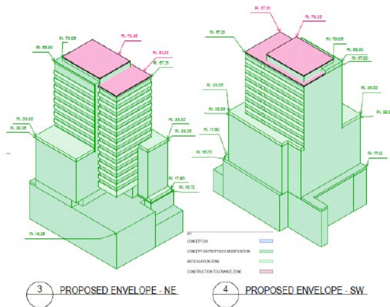
Figure 9: Proposed envelope (BVN)
