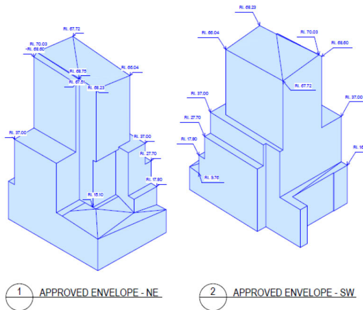
Figure 8: Approved envelope (BVN)
